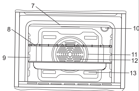
Four encastrable
